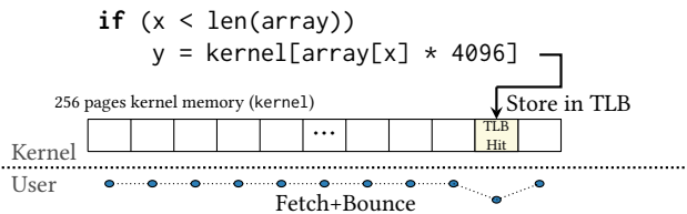
Figure 5: Speculative Fetch+Bounce allows an attacker to use Spectre gadgets to leak data from the kernel, by encoding them in the TLB.
